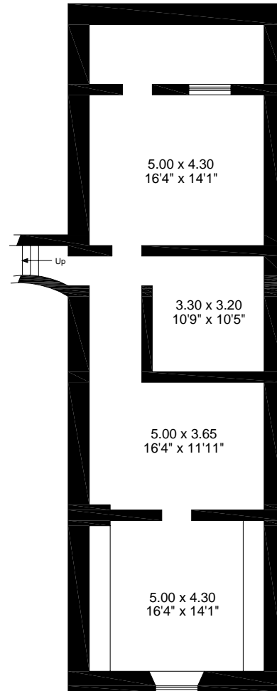
Cellar Plan
